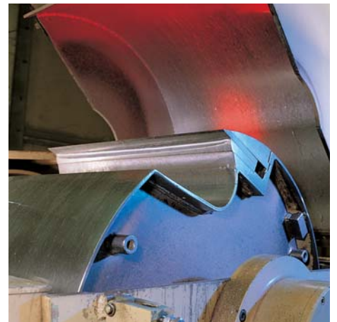
Detailed View Chipper Knives
